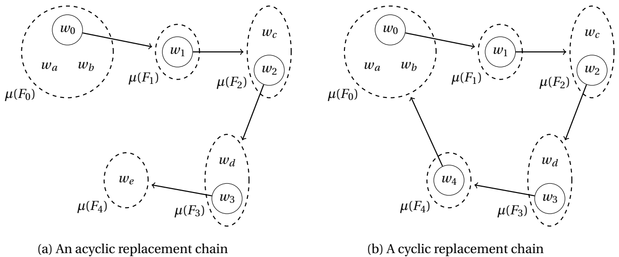
Figure 2: Two replacement chains
